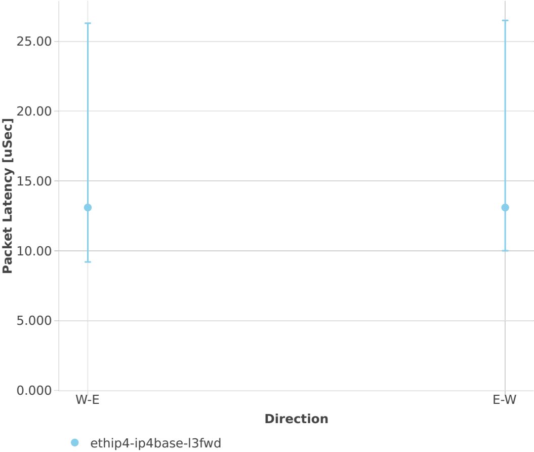
Latency: l3fwd-2n-skx-x710-64b-2t1c-base-ndr
