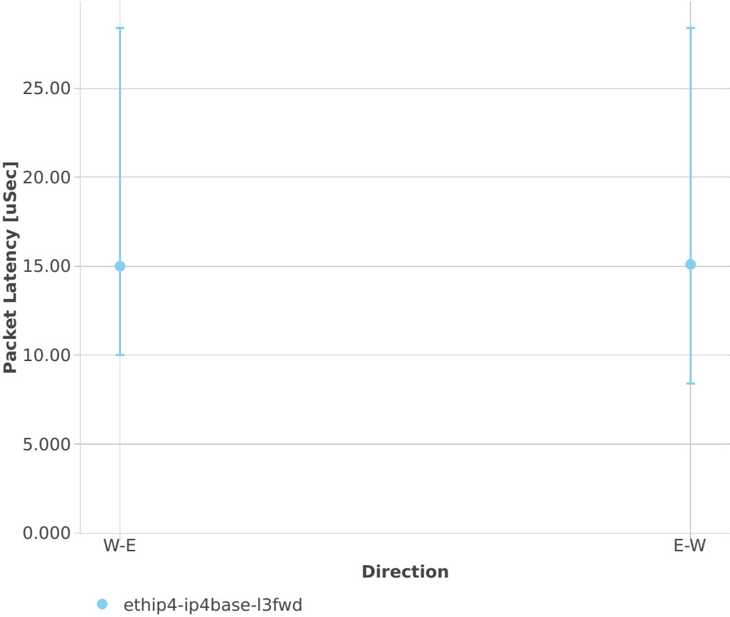
Latency: l3fwd-2n-skx-x710-64b-4t2c-base-ndr
