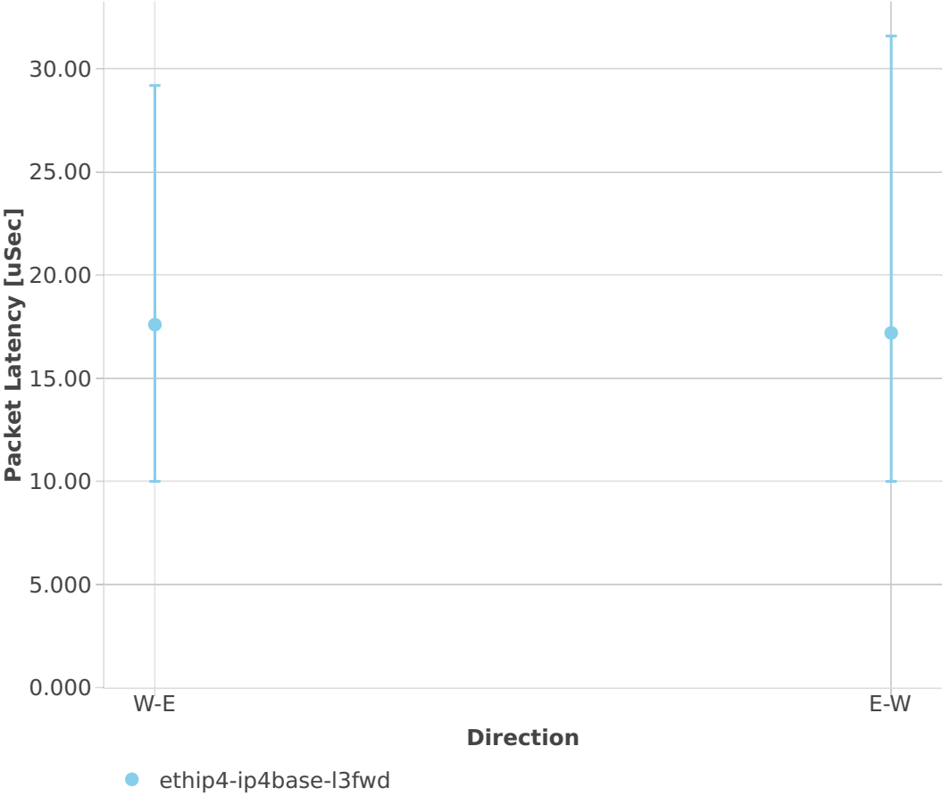
Latency: l3fwd-2n-skx-xxv710-64b-4t2c-base-ndr
