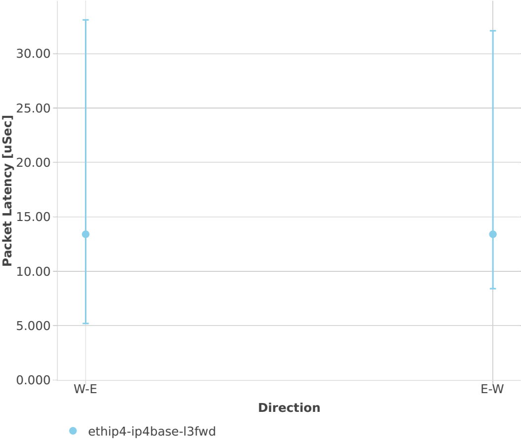
Latency: l3fwd-3n-hsw-x520-64b-1t1c-base-ndr
