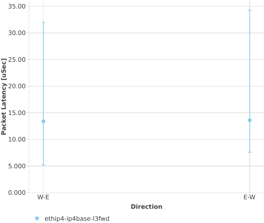
Latency: l3fwd-3n-hsw-x520-64b-2t2c-base-ndr
