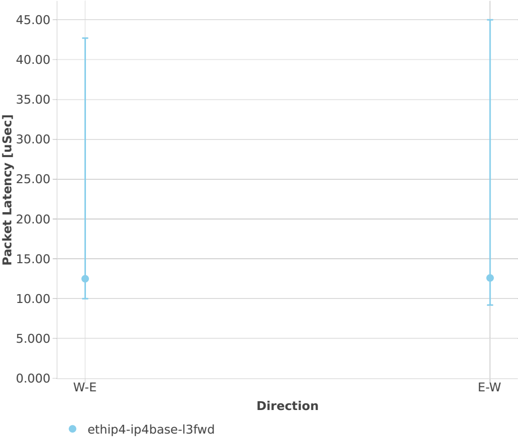
Latency: l3fwd-3n-hsw-x710-64b-1t1c-base-ndr
