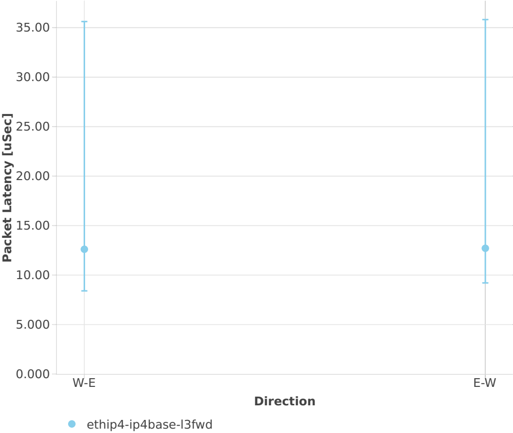
Latency: l3fwd-3n-hsw-x710-64b-2t2c-base-ndr
