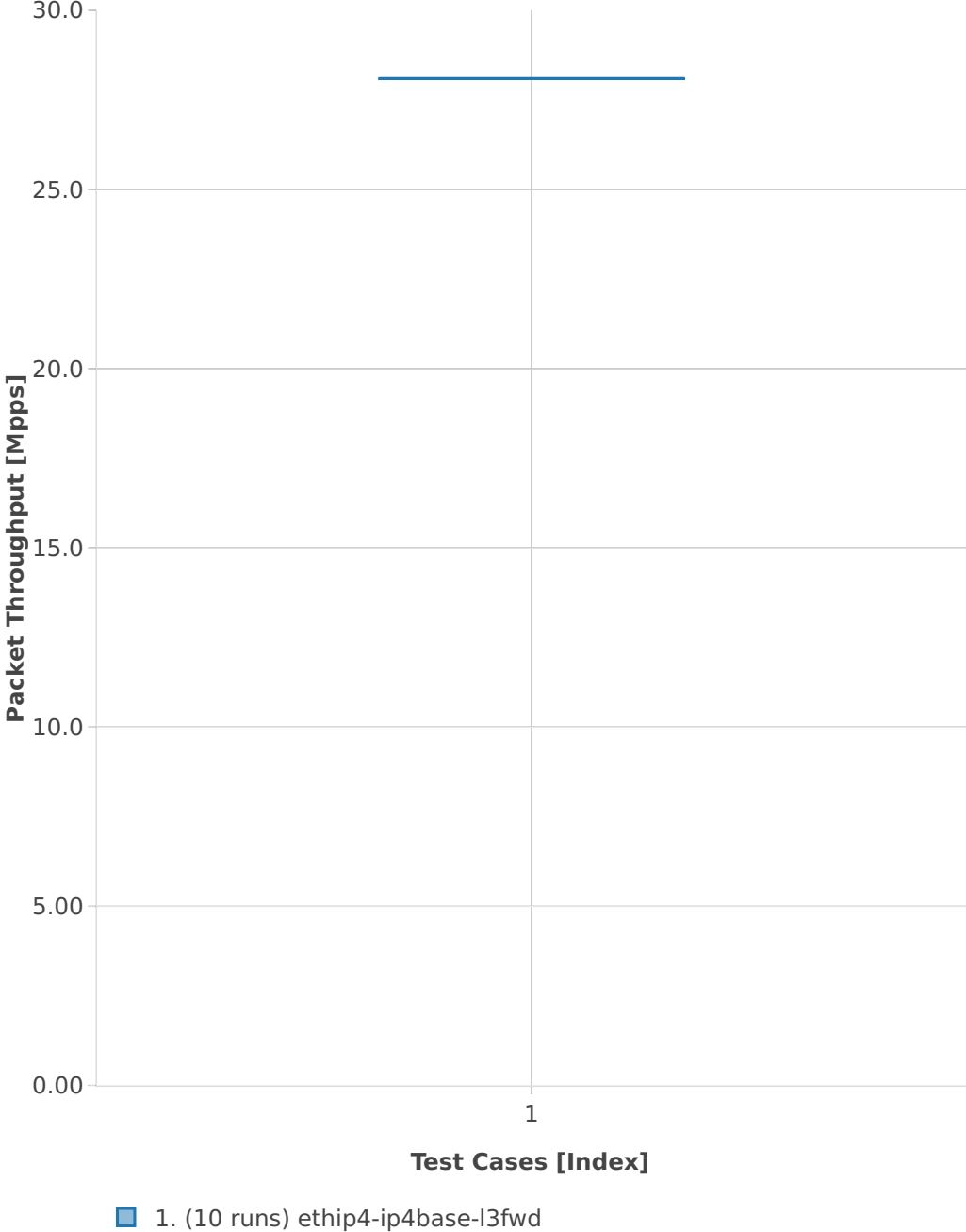
Throughput: l3fwd-3n-hsw-x710-64b-2t2c-base-pdr
