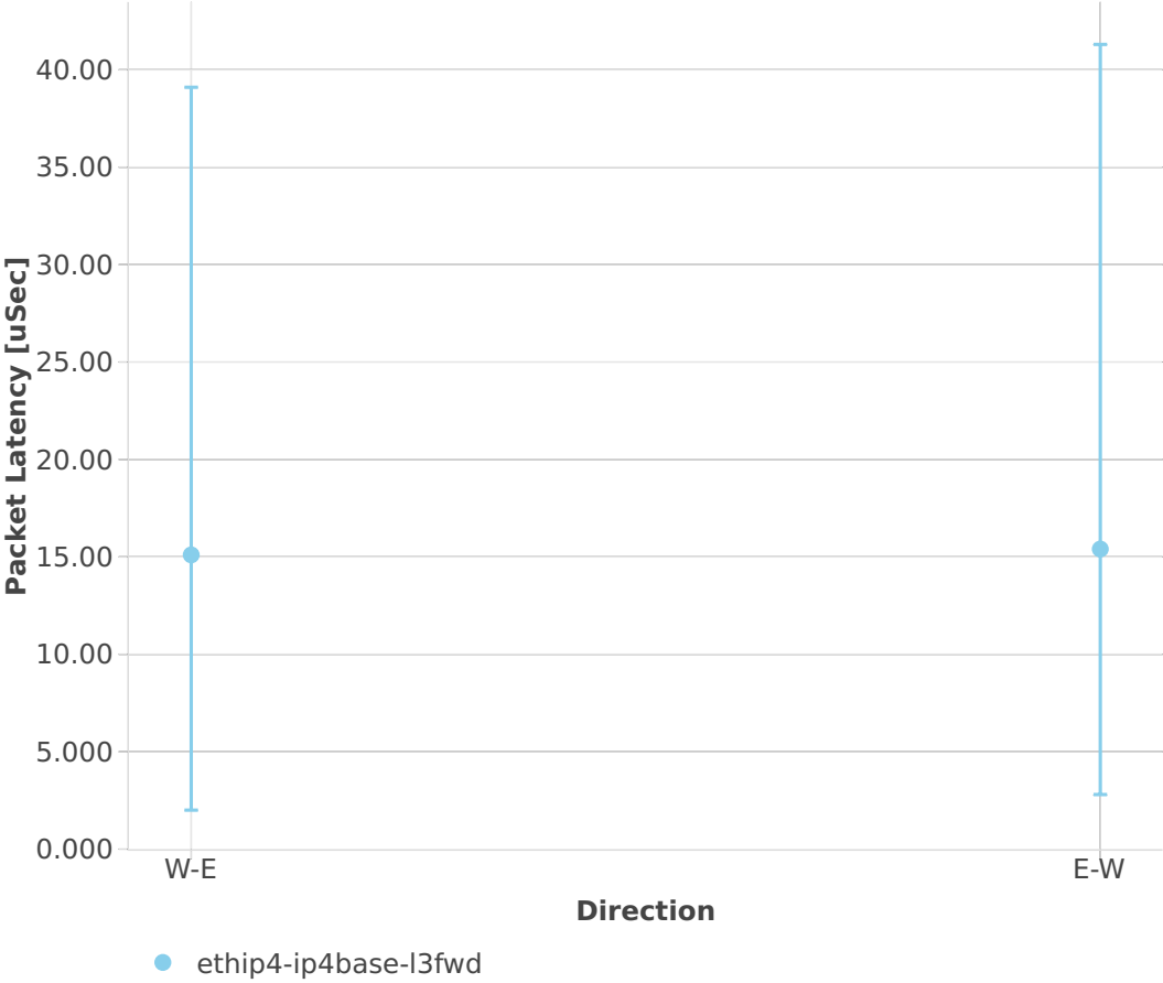
Latency: l3fwd-3n-hsw-xl710-64b-1t1c-base-ndr
