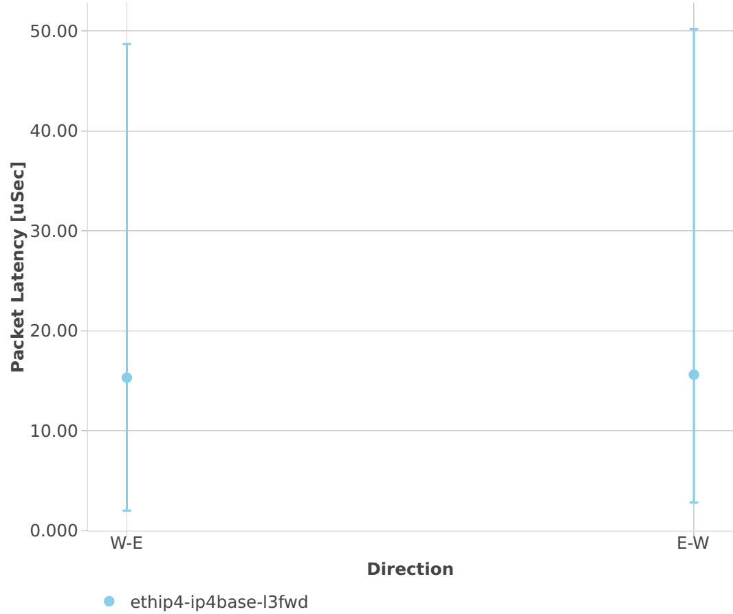
Latency: l3fwd-3n-hsw-xl710-64b-2t2c-base-ndr
