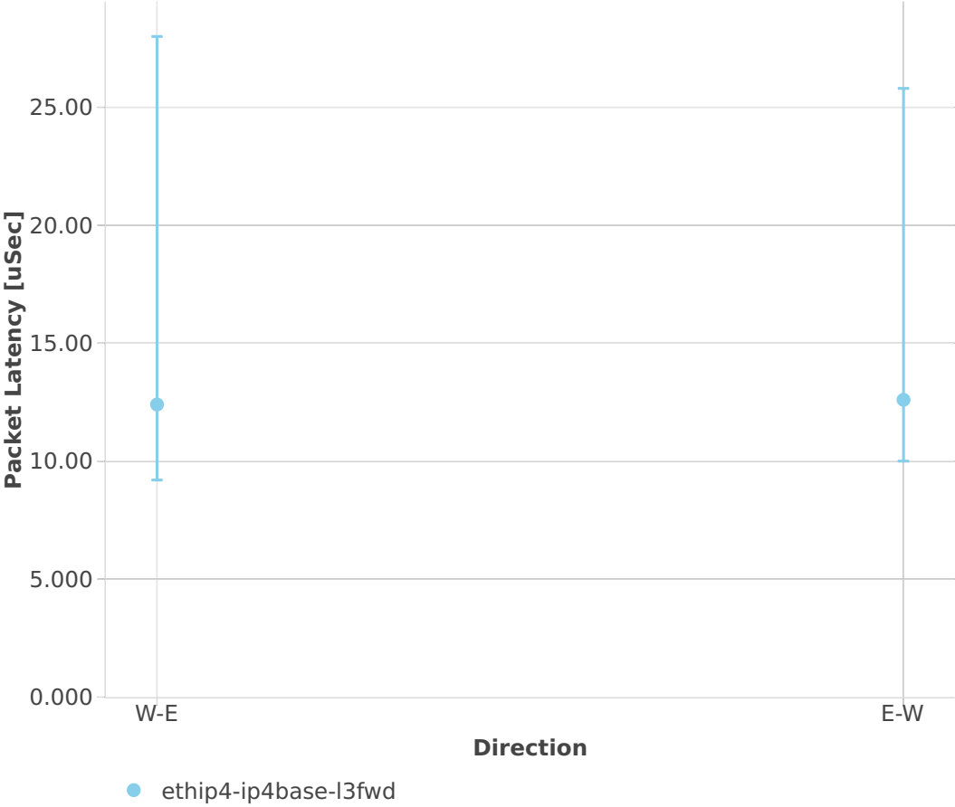
Latency: l3fwd-3n-skx-x710-64b-2t1c-base-ndr
