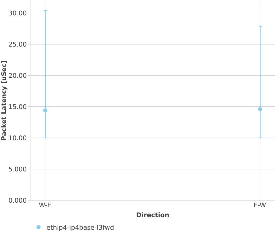
Latency: l3fwd-3n-skx-x710-64b-4t2c-base-ndr
