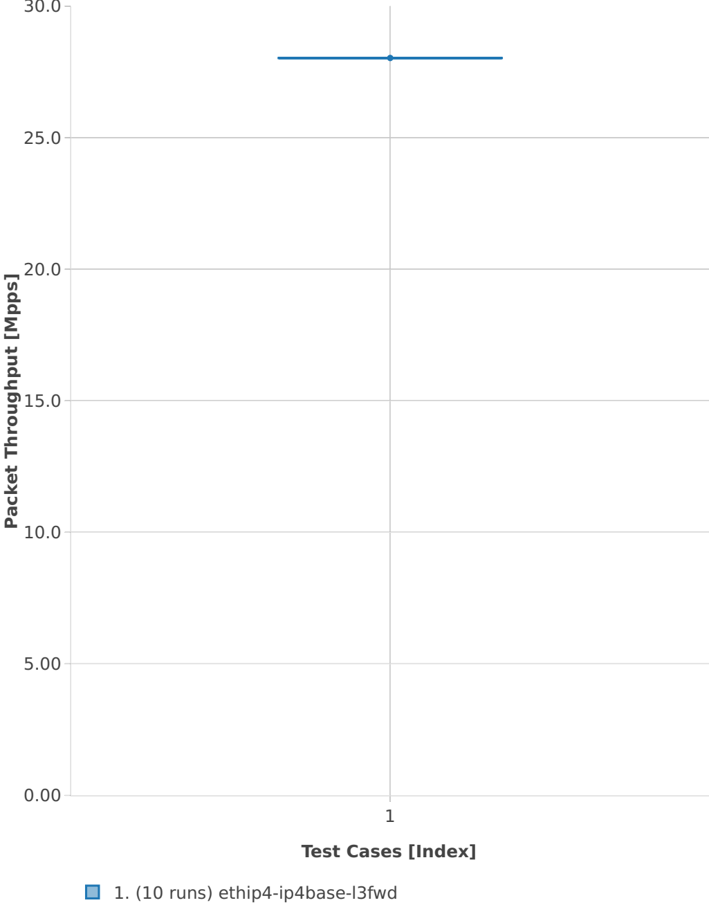
Throughput: l3fwd-3n-skx-x710-64b-4t2c-base-pdr
