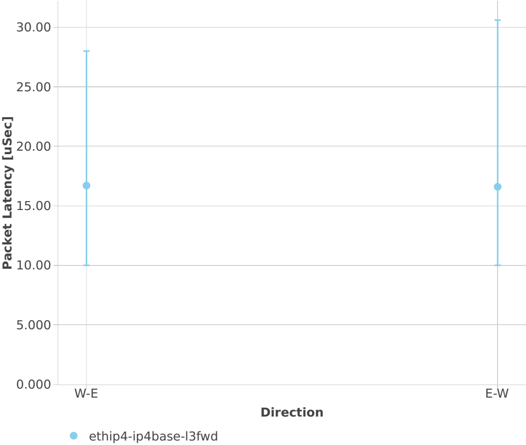
Latency: l3fwd-3n-skx-xxv710-64b-4t2c-base-ndr
