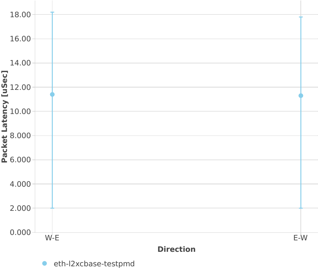
Latency: testpmd-2n-skx-x710-64b-2t1c-base-ndr
