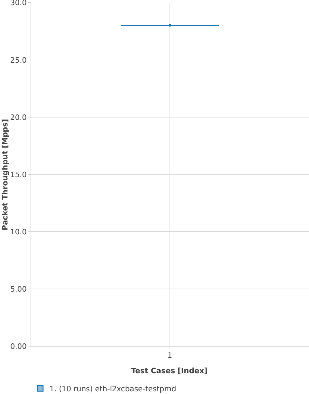
Throughput: testpmd-2n-skx-x710-64b-2t1c-base-pdr
