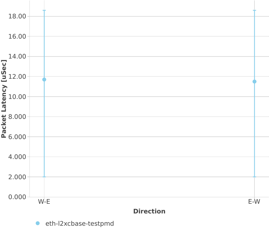
Latency: testpmd-2n-skx-x710-64b-4t2c-base-ndr
