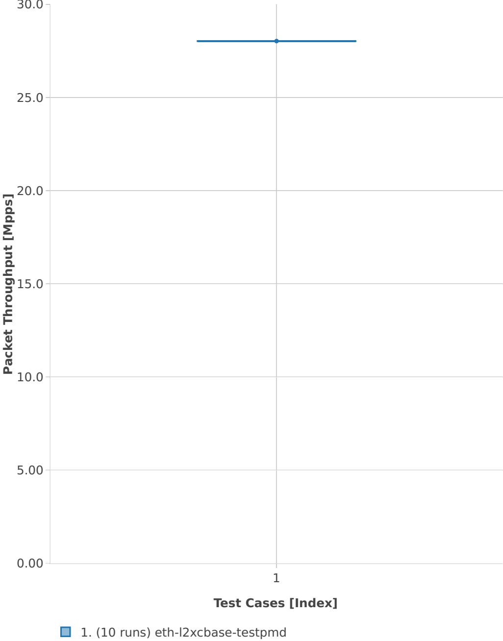
Throughput: testpmd-2n-skx-x710-64b-4t2c-base-pdr
