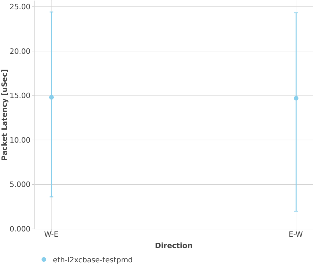
Latency: testpmd-2n-skx-xxv710-64b-2t1c-base-ndr
