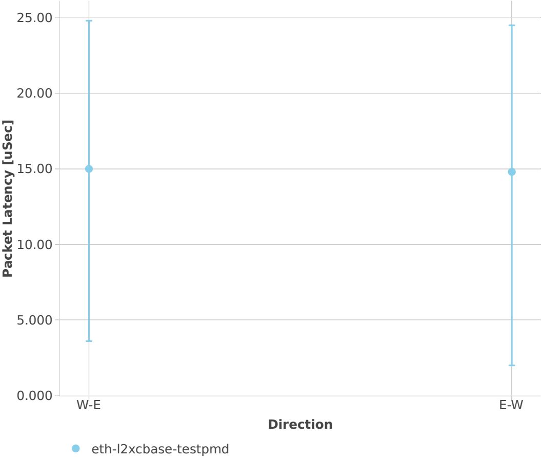
Latency: testpmd-2n-skx-xxv710-64b-4t2c-base-ndr
