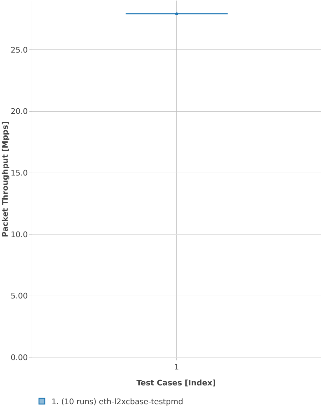
Throughput: testpmd-2n-skx-xxv710-64b-4t2c-base-pdr
