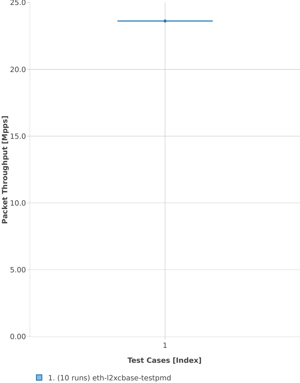
Throughput: testpmd-3n-hsw-x520-64b-1t1c-base-ndr
