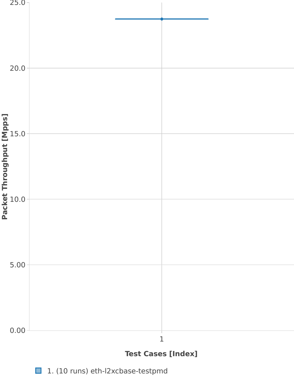
Throughput: testpmd-3n-hsw-x520-64b-1t1c-base-pdr
