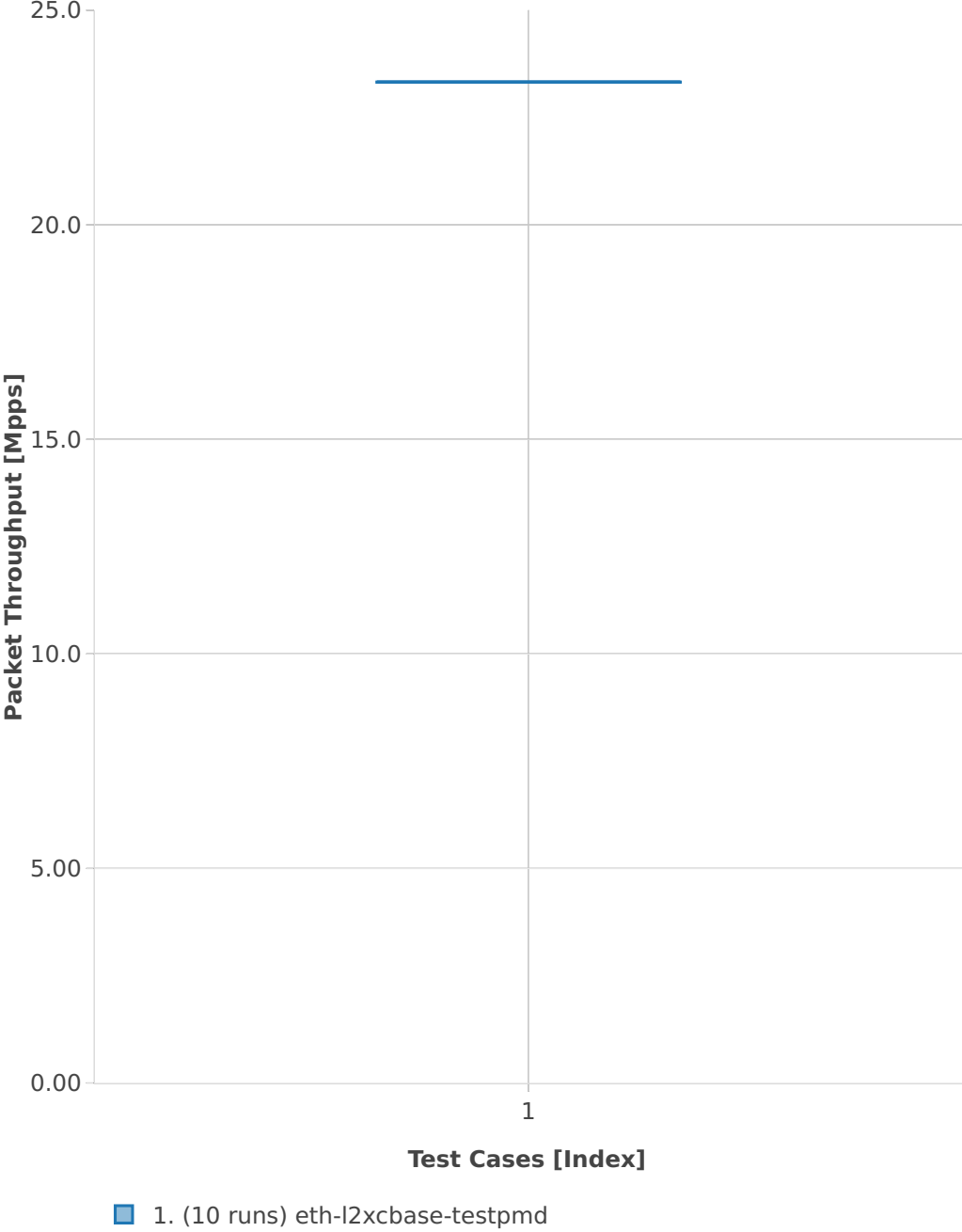
Throughput: testpmd-3n-hsw-x520-64b-2t2c-base-ndr
