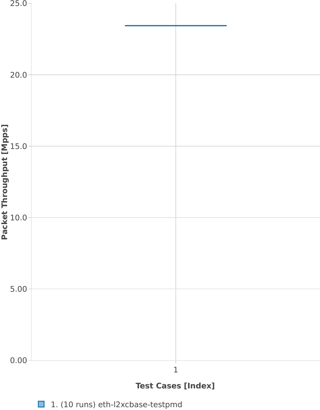
Throughput: testpmd-3n-hsw-x520-64b-2t2c-base-pdr
