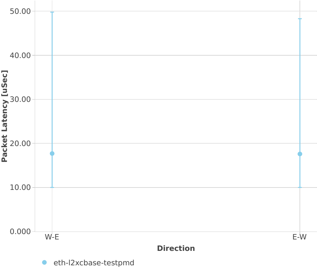
Latency: testpmd-3n-hsw-x710-64b-2t2c-base-ndr
