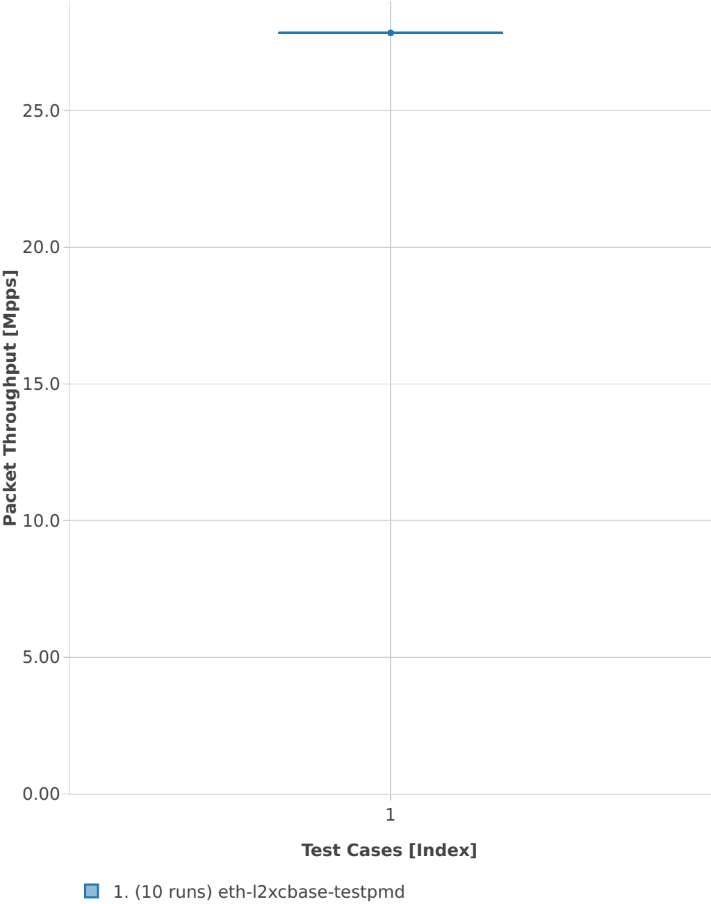
Throughput: testpmd-3n-hsw-x710-64b-2t2c-base-ndr
