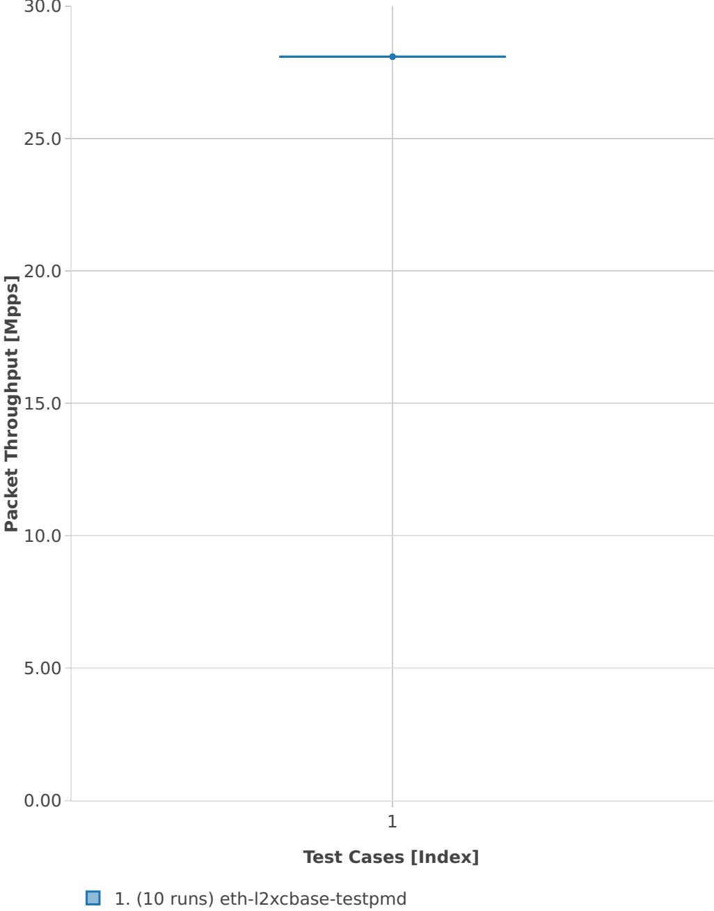
Throughput: testpmd-3n-hsw-x710-64b-2t2c-base-pdr
