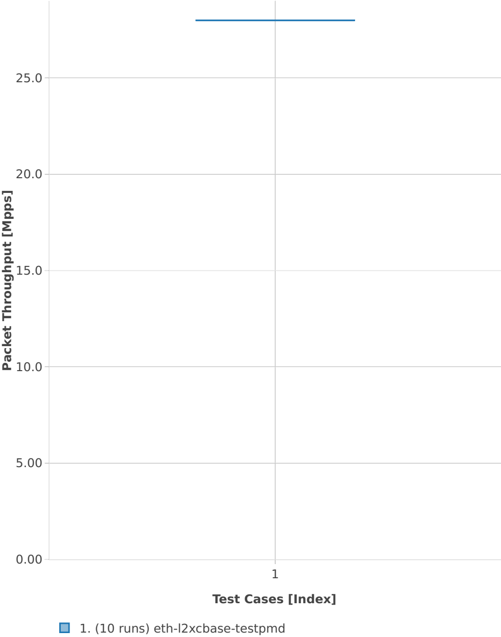
Throughput: testpmd-3n-hsw-xl710-64b-1t1c-base-pdr
