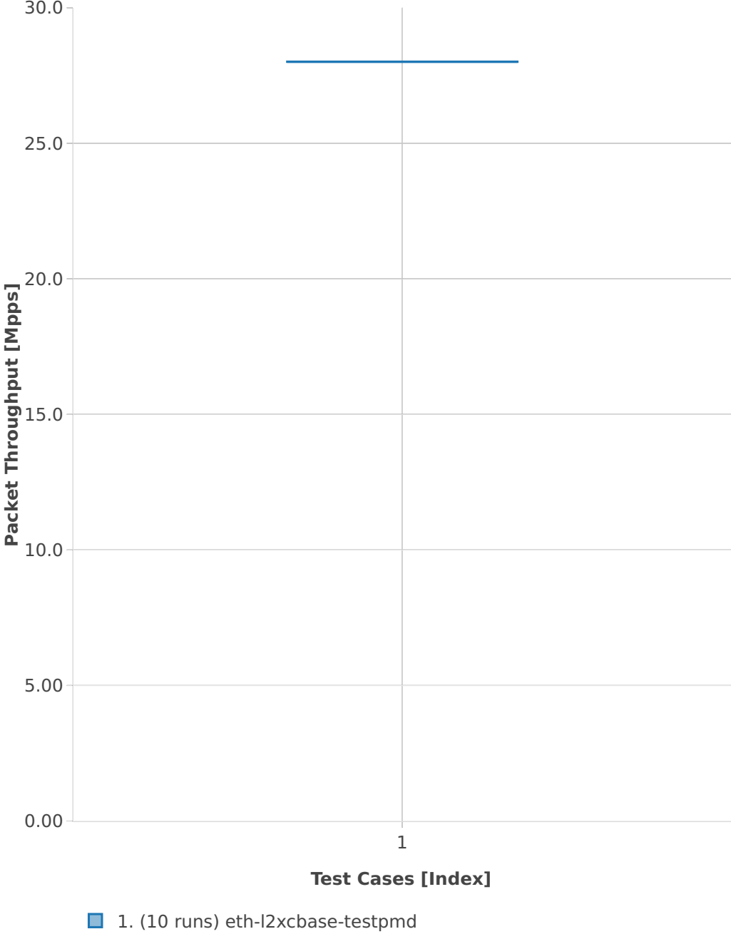
Throughput: testpmd-3n-hsw-xl710-64b-2t2c-base-pdr
