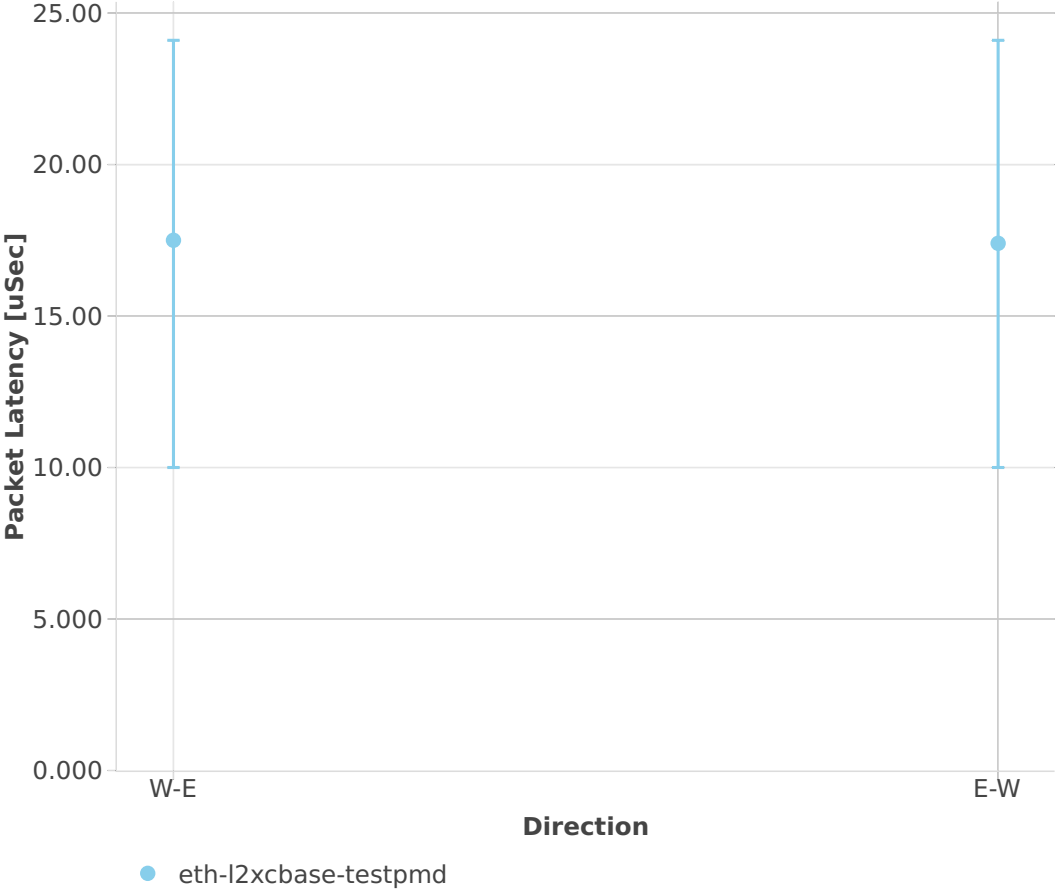
Latency: testpmd-3n-skx-x710-64b-2t1c-base-ndr
