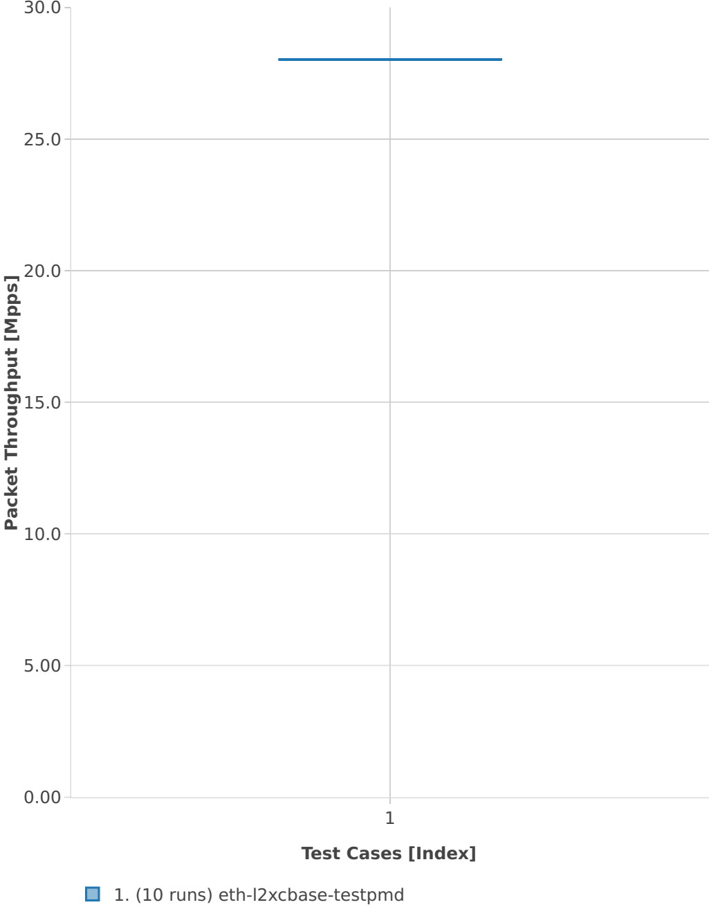
Throughput: testpmd-3n-skx-x710-64b-2t1c-base-pdr
