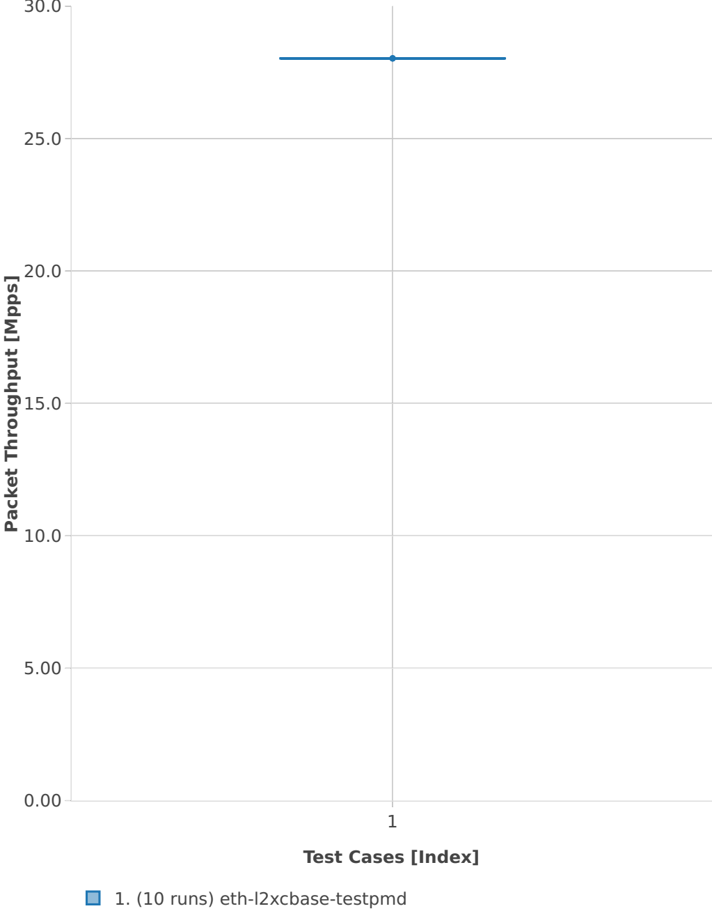
Throughput: testpmd-3n-skx-x710-64b-4t2c-base-pdr
