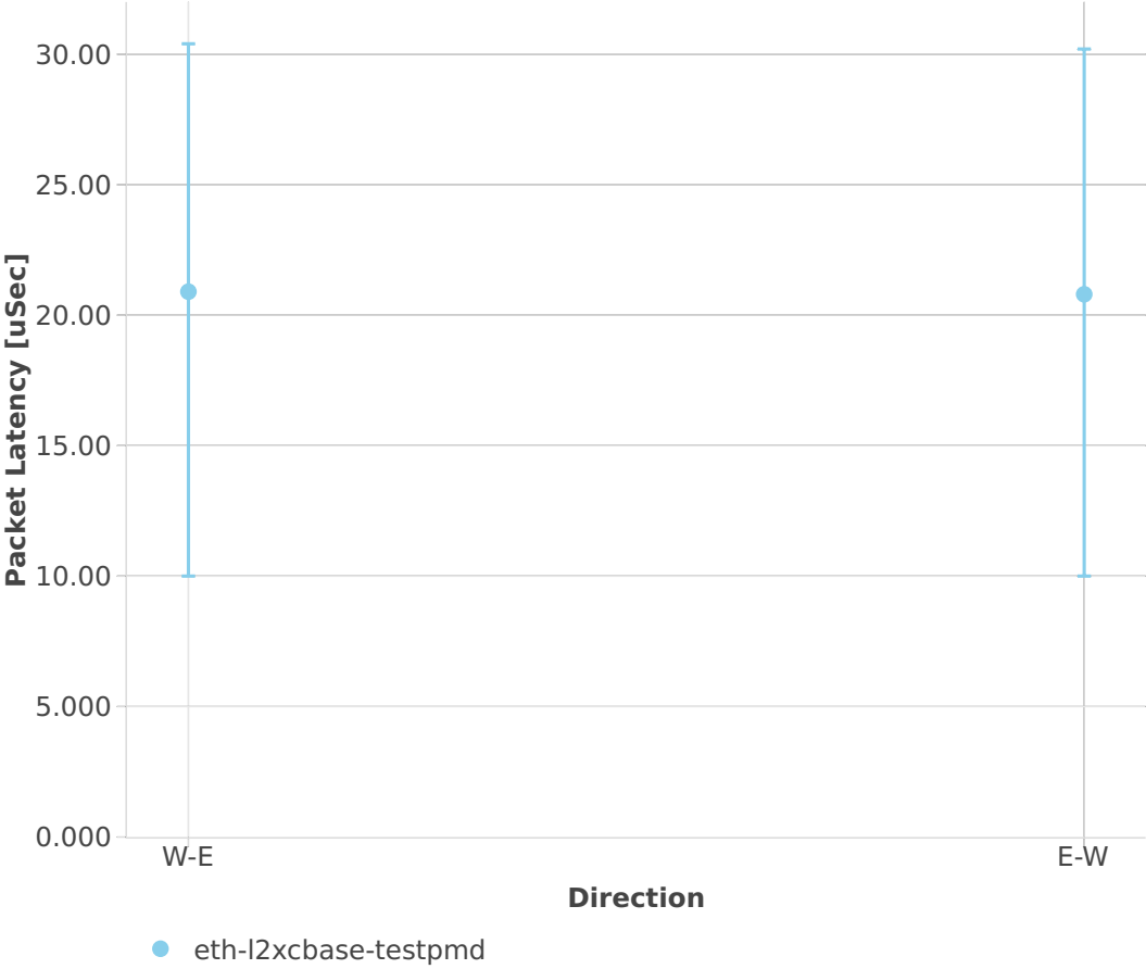
Latency: testpmd-3n-skx-xxv710-64b-2t1c-base-ndr
